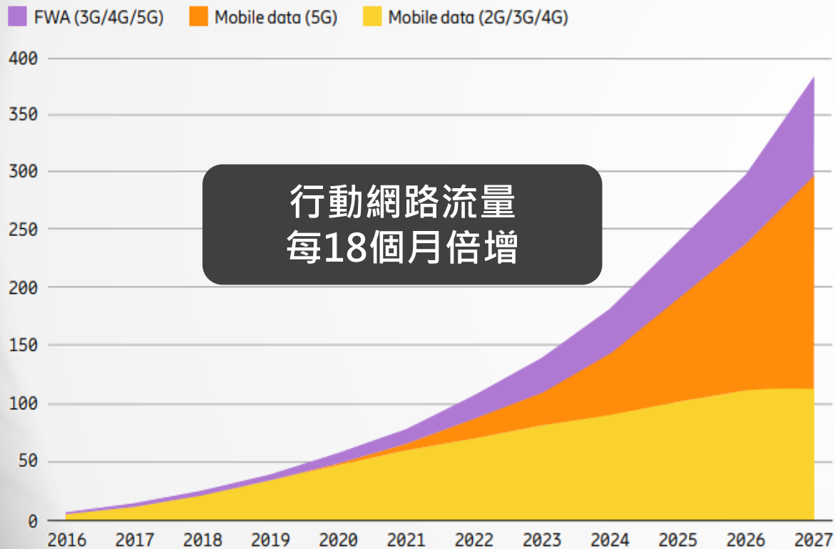
Figure 18: Global mobile network data traffic (EB per month)
